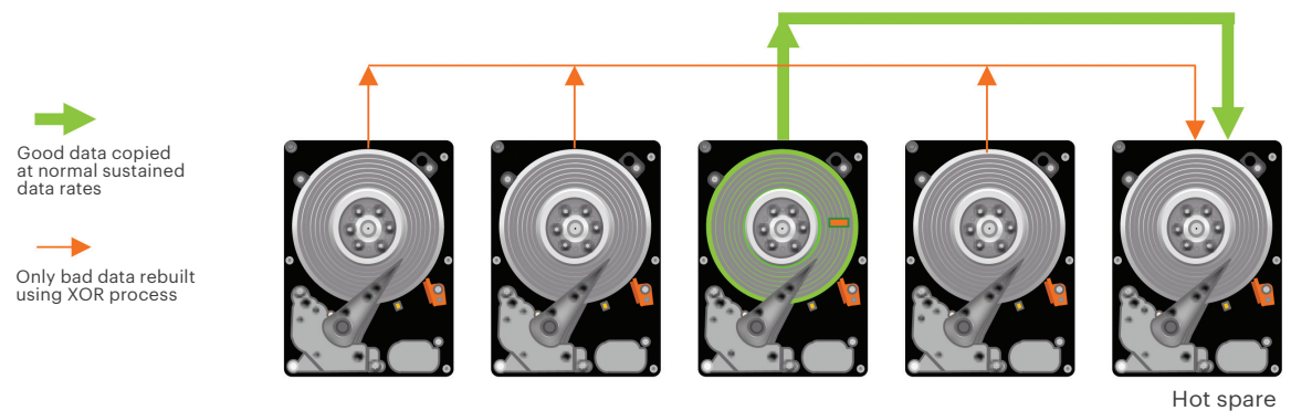
Figure 2. Rebuild Assist quickly copies the good data from the drive with errors. It then reconstructs the missing data using the remaining healthy drives, significantly reducing rebuild times.
