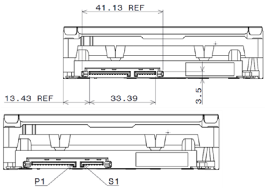
Figure 8 Connector locations
