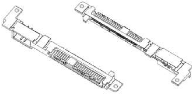
Figure 3 SAS Connector
