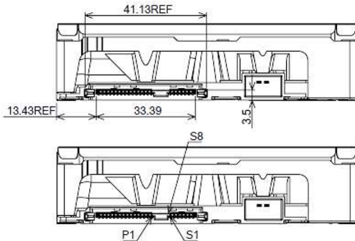
Figure 9 Connector locations
