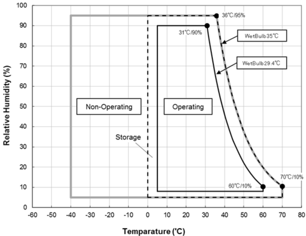
Figure 6 Limits of temperature and humidity
