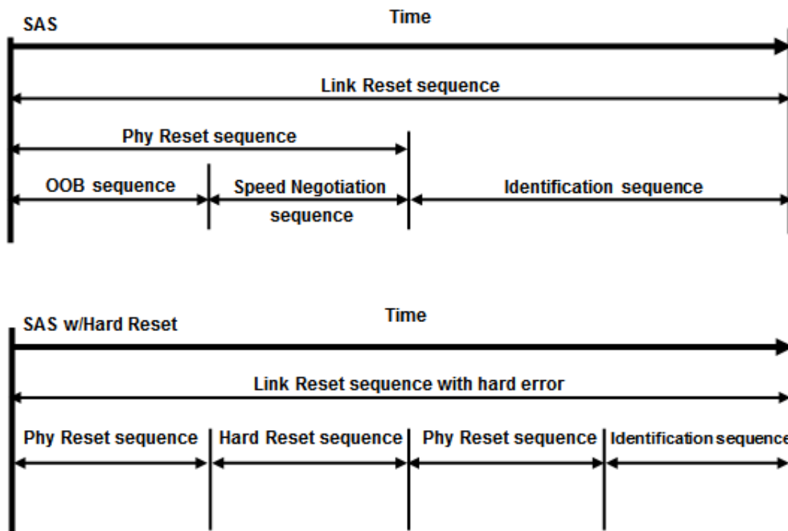
Figure 11 Link Reset Sequence
