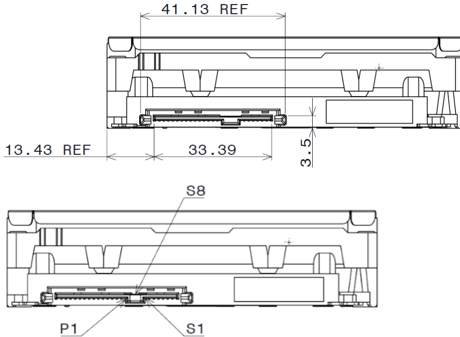
Figure 9 Connector locations
