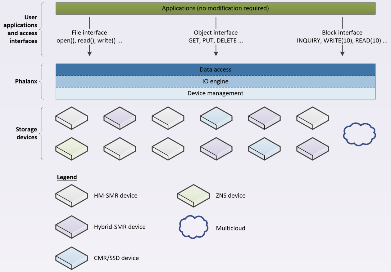
Figure 2 - Phalanx software stack
