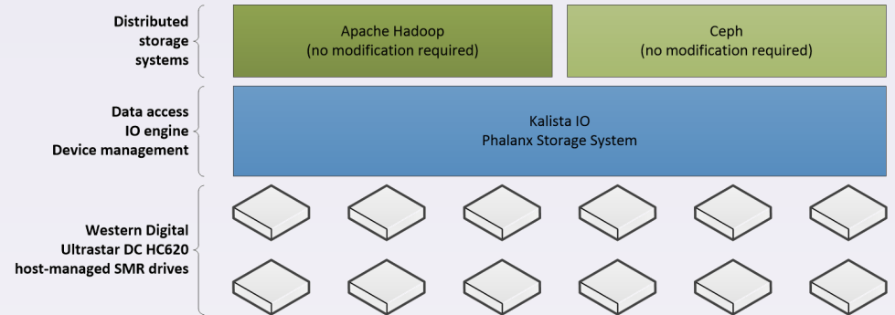
Figure 4 - Enabling Apache Hadoop and Ceph with Western Digital's Ultrastar DC HC620 host-managed SMR drives
