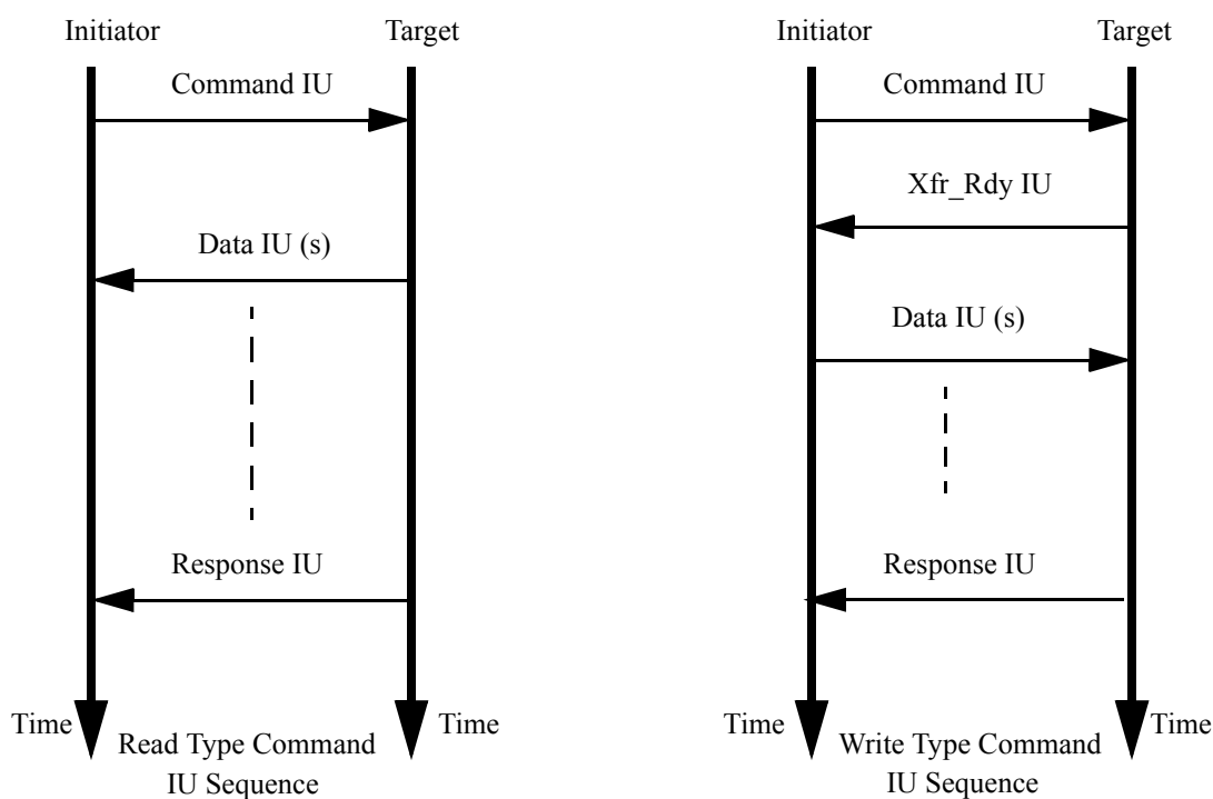
Figure 1: SSP Information Unit Sequences
