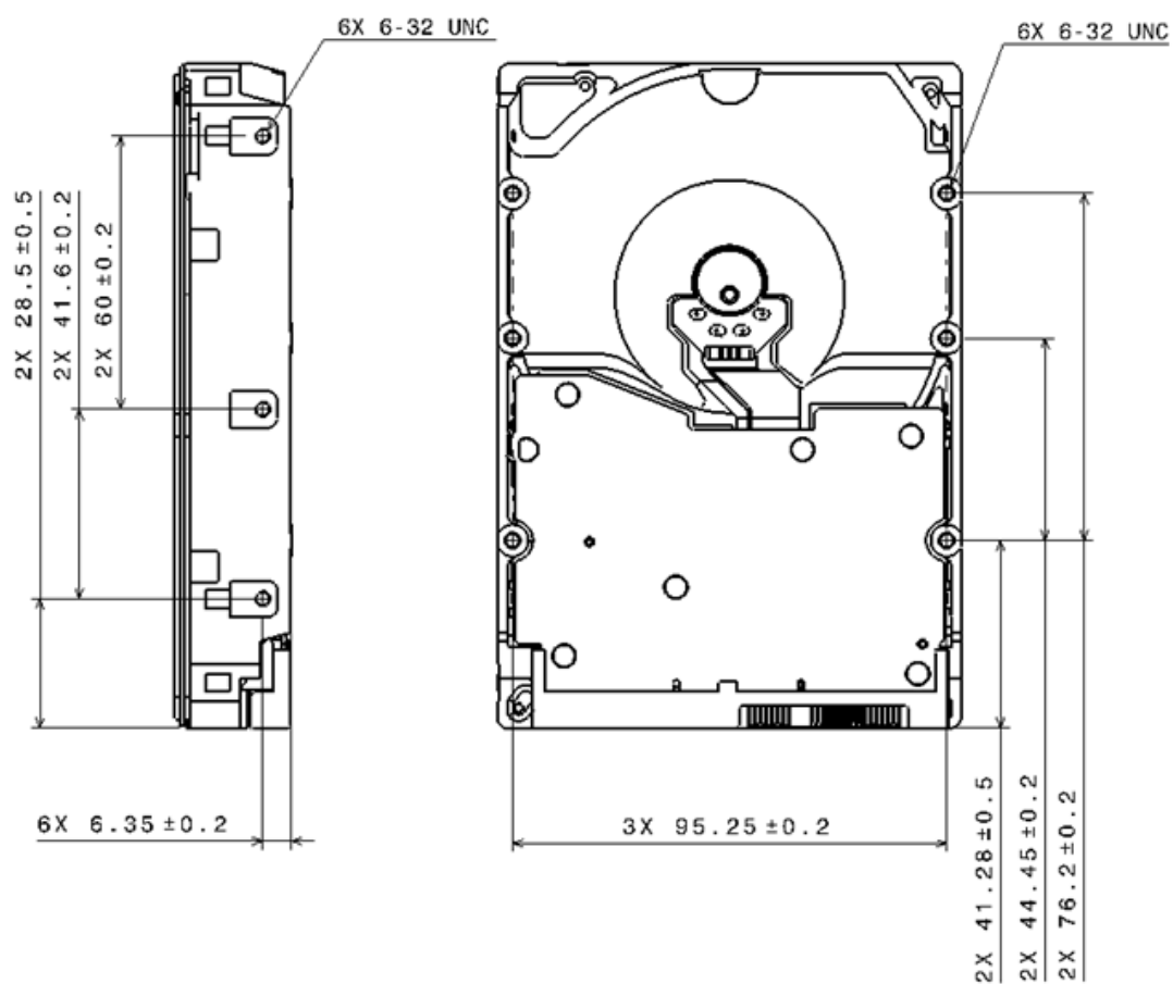
Figure 8 Bottom and side views with mounting hole locations
