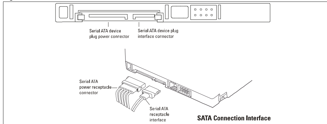
Figure 5-2. Connector Locations
