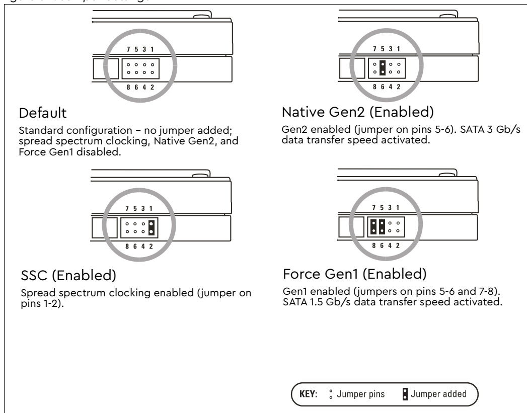
Figure 5-1. Jumper Settings
