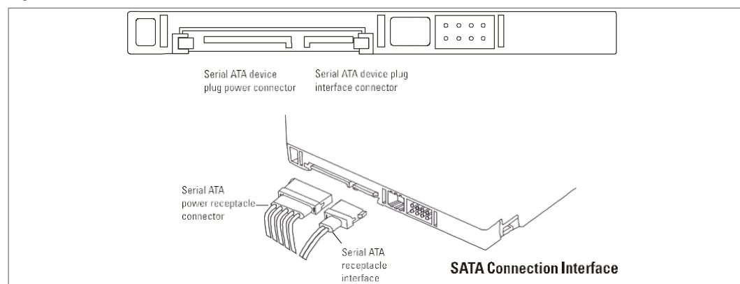
Figure 5-1. Connector Locations
