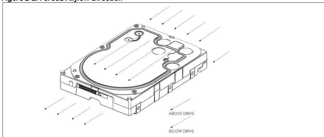
Figure 2-2. Forced Airflow Direction
