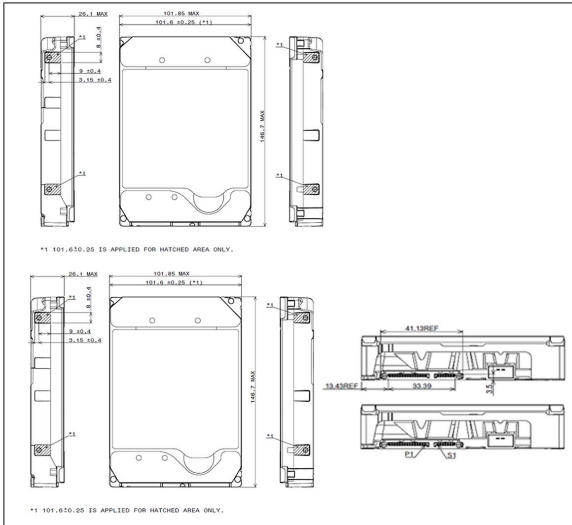
Figure 2-1. Mounting Dimensions
