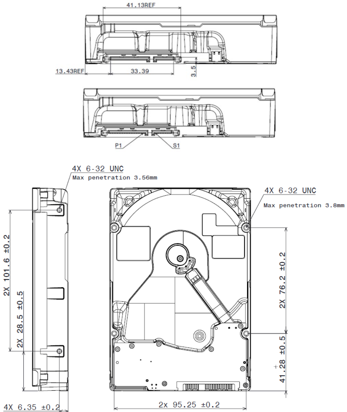
Figure 1 Mounting Dimensions
